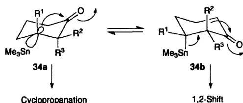
Scheme 9.
